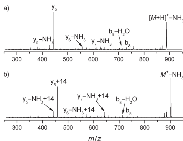
Figure 3. ESI-MS/MS spectra of a) y 9 + (905.48 Da) and b) [y 9 + 14] + (919.47 Da).
